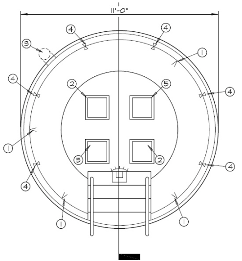
WHIRLPOOL PLAN VIEW SCALE: 3/8" = 1'-0"
